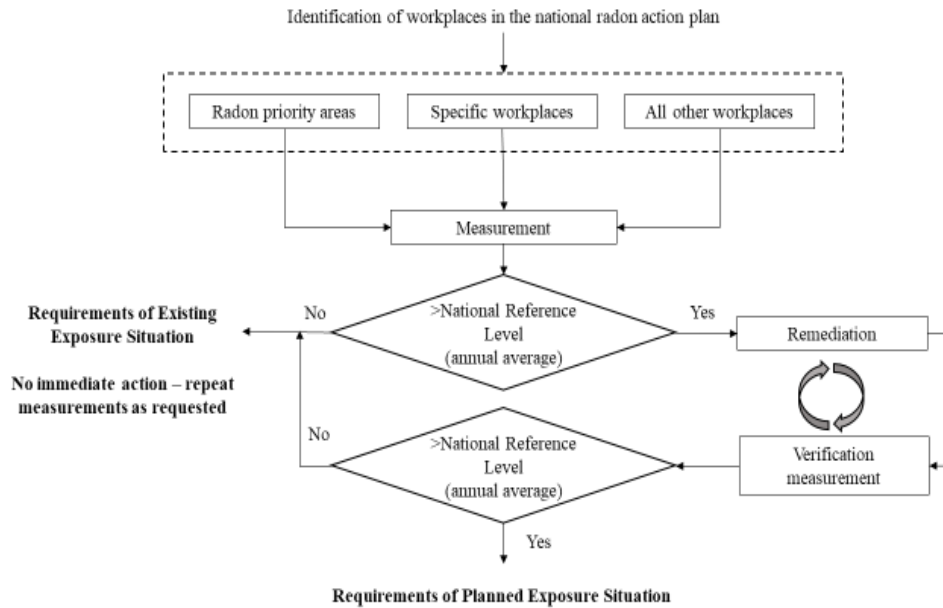
FIG. 2 Flow chart illustrating how to select approach for protection of workers against radon exposure based on the annual average activity concentration of ^{222}\text{Rn} in air in workplaces.
