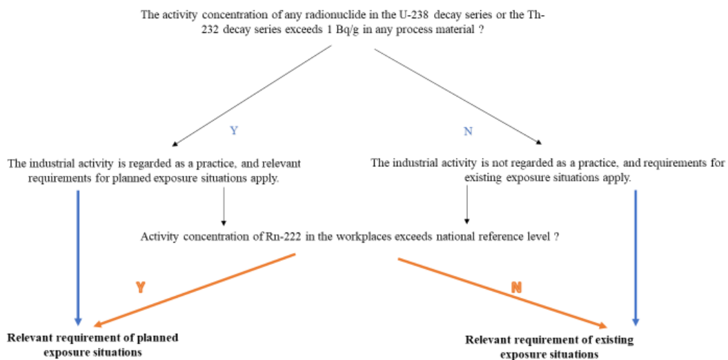
FIG. 1. Flow chart illustrating how to select approach for protection of workers against radon exposure based either on the activity concentration in material of uranium or thorium decay series or activity concentration of radon.
