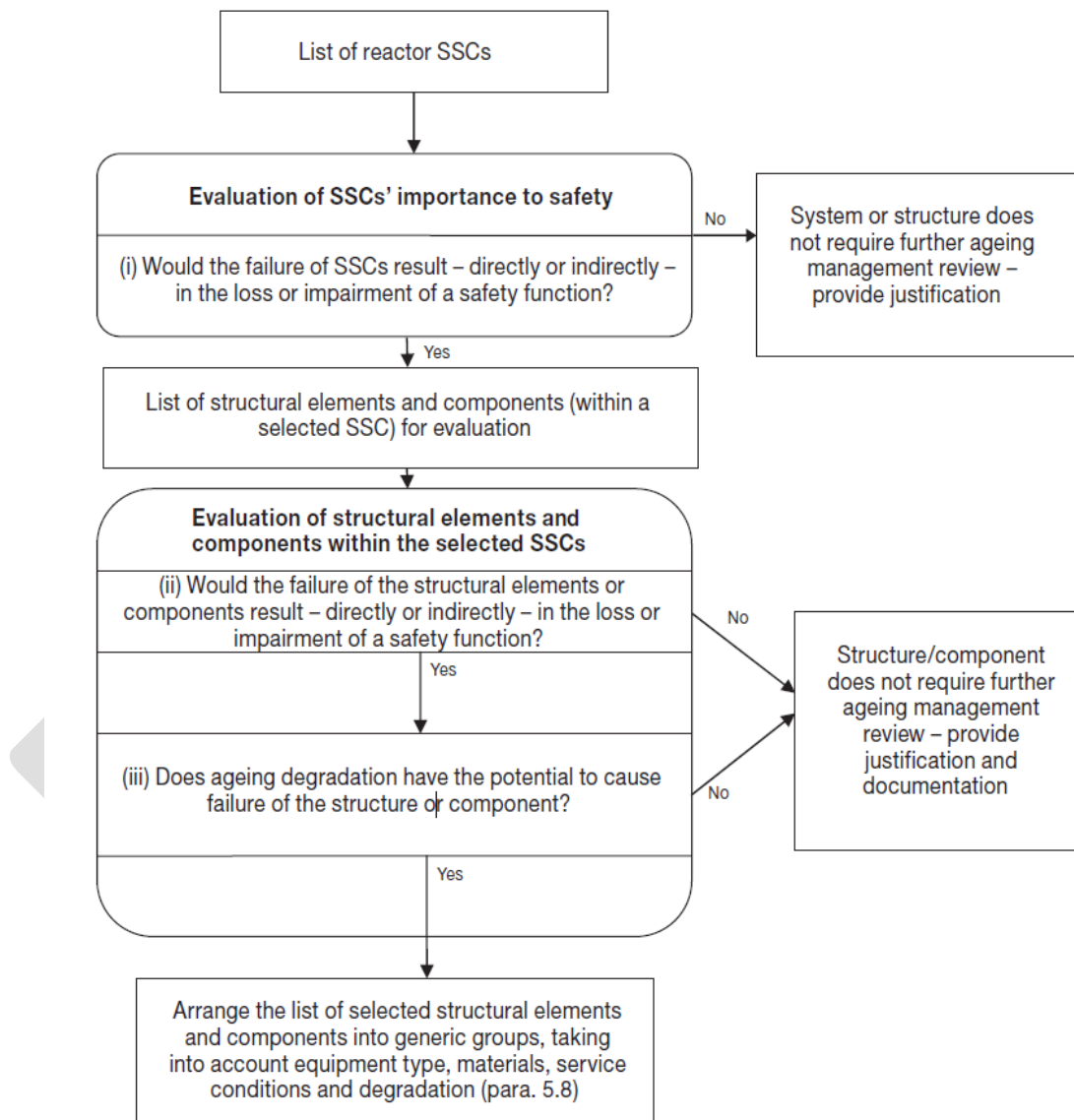
FIG 1. Outline of the process for screening SSCs for ageing management.
