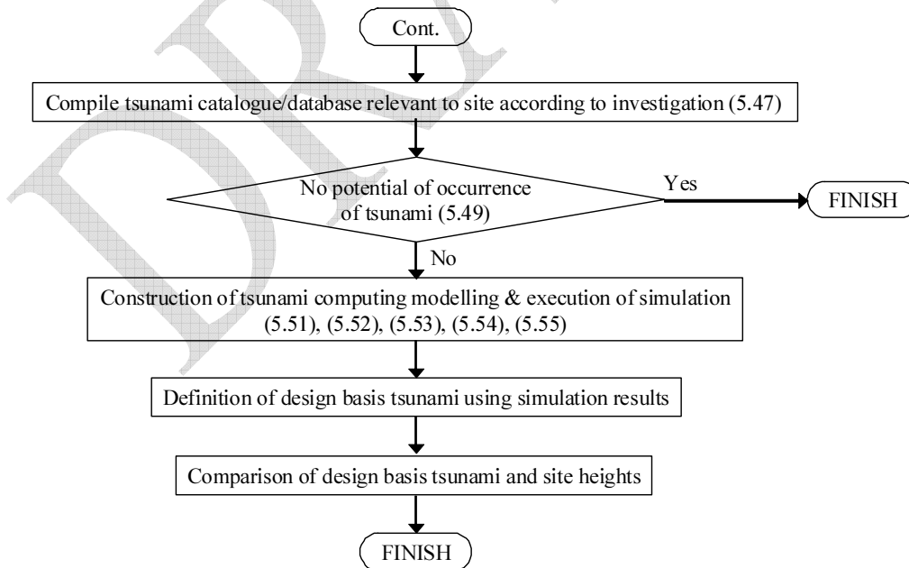
Figure 1 Flowchart of initial and detailed assessment of tsunami flooding
