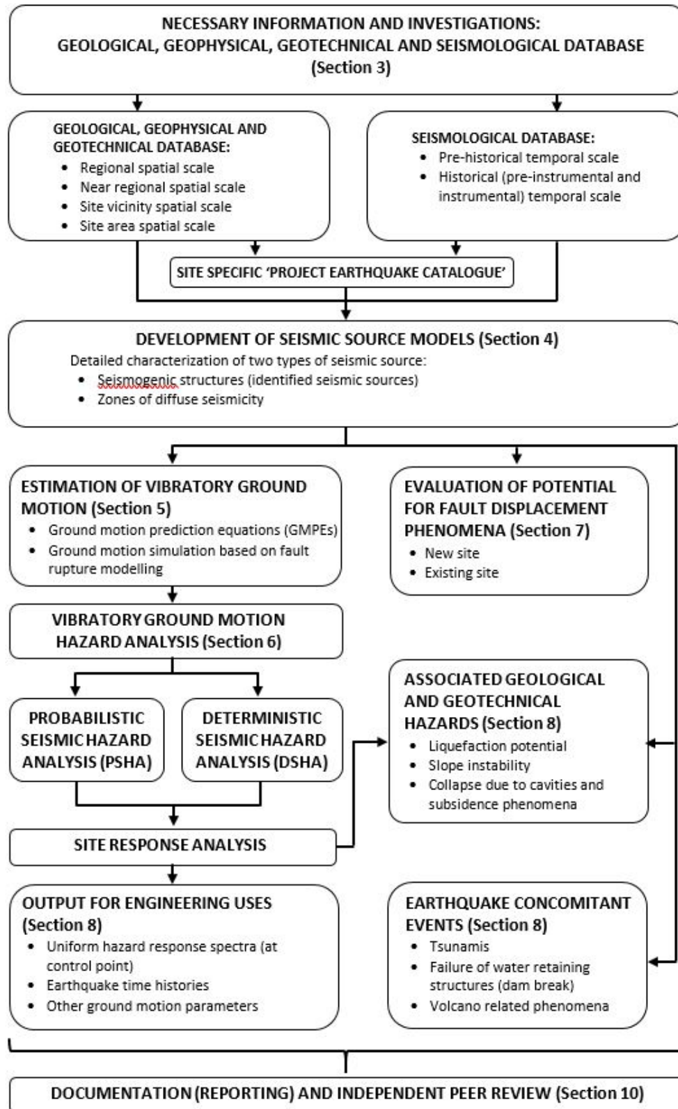
FIG. 1:- Flow chart for showing the seismic hazard assessment process for nuclear installations.
