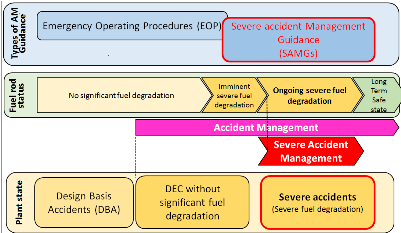
Figure 1.FIG. 3. Comparison of Relationship between the Fuel Status, and Accident the plant State to and the type of a Accident Management guidance Domain.
