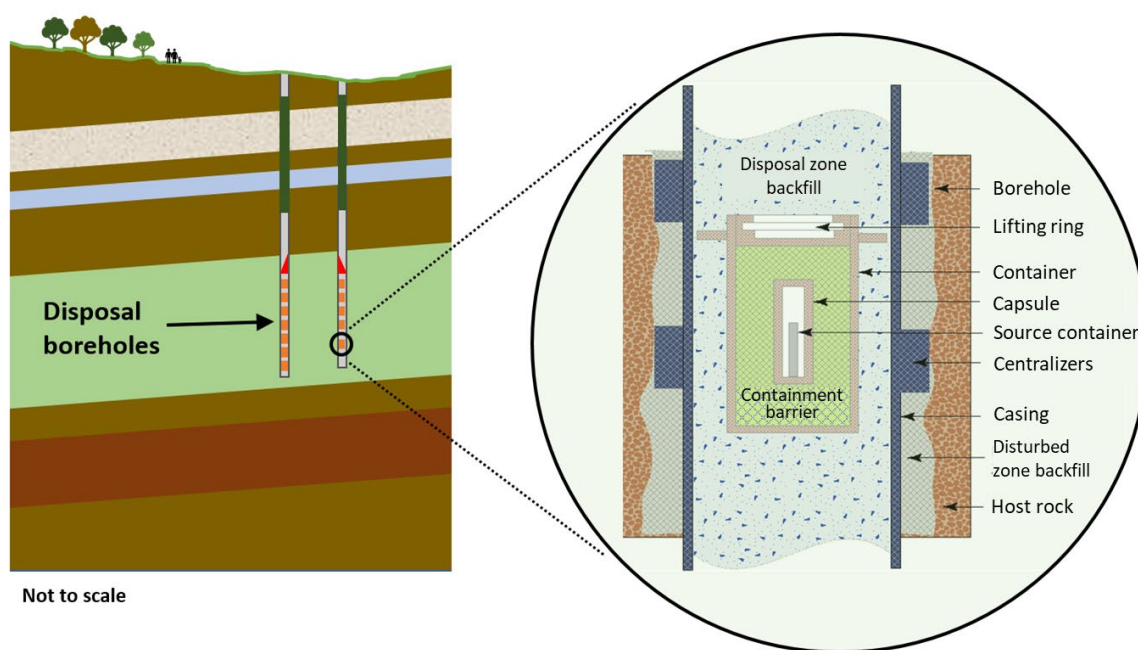
FIG. 1. Example of a borehole disposal system for disused sealed radioactive sources.
