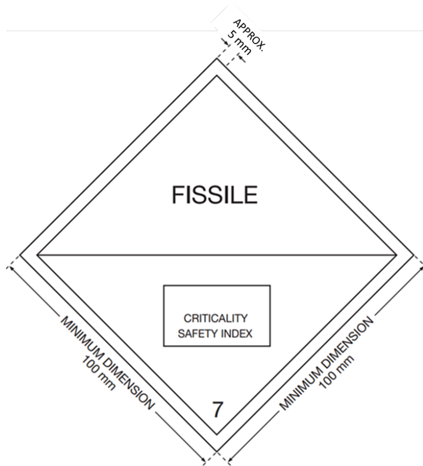
FIG. 5. CSI label. The background colour of the label shall be white, the colour of the printing shall be black.
