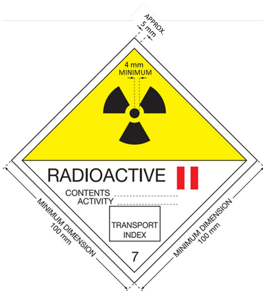
FIG. 3. Category II-YELLOW label. The background colour of the upper half of the label shall be yellow and the lower half white, the colour of the trefoil and the printing shall be black, and the colour of the category bars shall be red.
