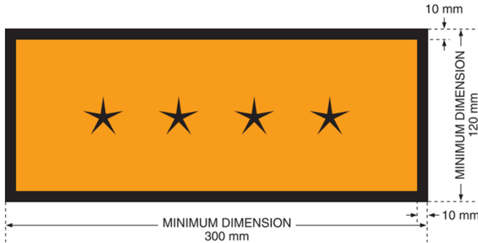
FIG. 7. Placard for separate display of UN number. The background colour of the placard shall be orange and the border and UN number shall be black. The symbol “★ ★ ★ ★” denotes the space in which the appropriate UN number for radioactive material, as specified in Table 1, shall be displayed.
