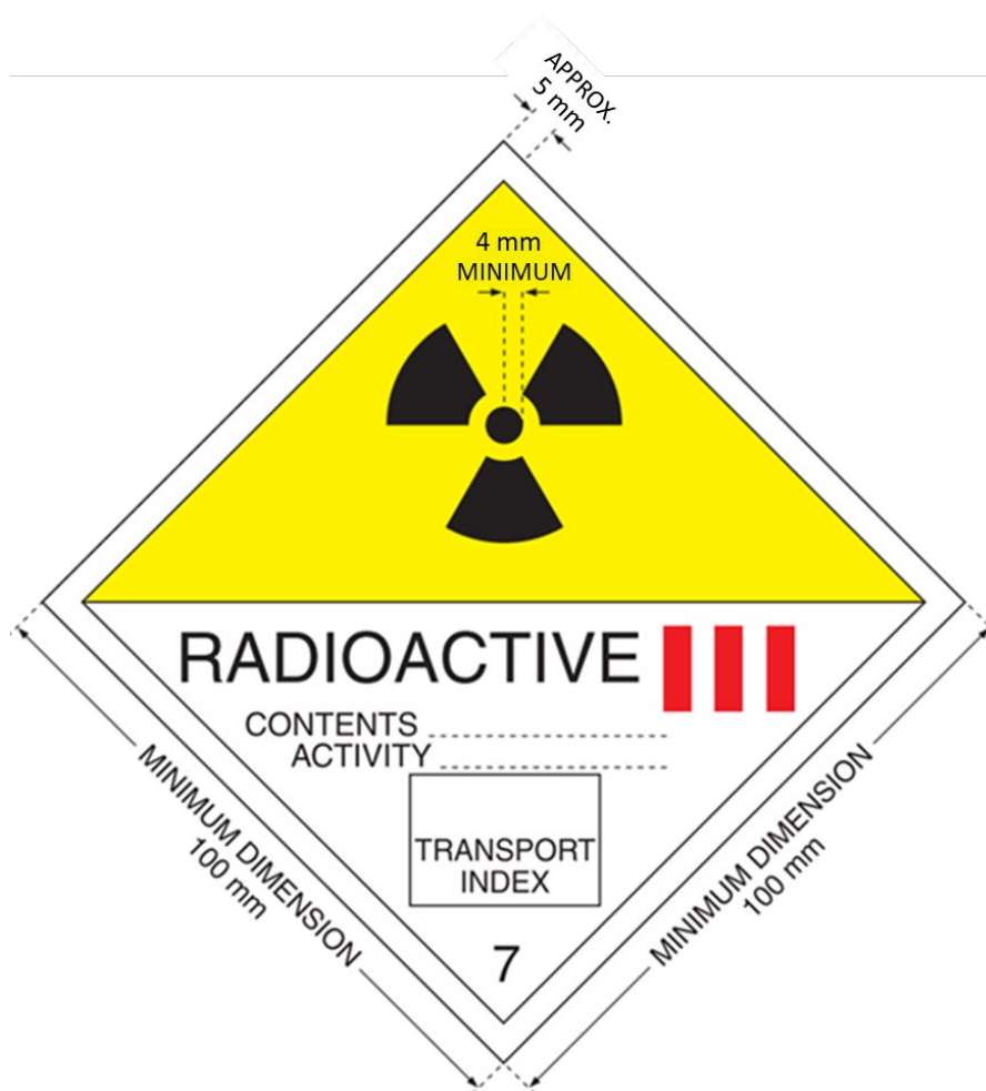
FIG. 4. Category III-YELLOW label. The background colour of the upper half of the label shall be yellow and the lower half white, the colour of the trefoil and the printing shall be black, and the colour of the category bars shall be red.
