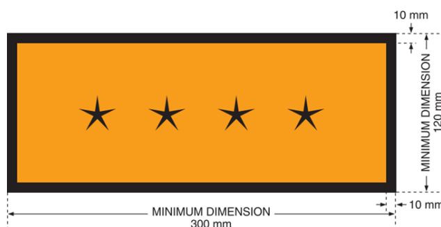
FIG. 7. Placard for separate display of UN number. The background colour of the placard shall be orange and the border and UN number shall be black. The symbol “★ ★ ★ ★ ****” denotes the space in which the appropriate UN number for radioactive material, as specified in Table 1, shall be displayed.
