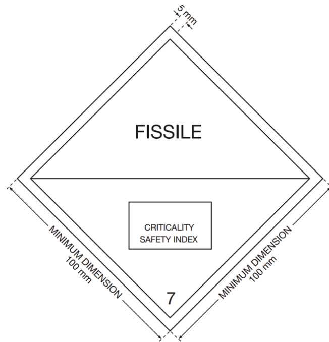
FIG. 5. CSI label. The minimum width of the line inside the edge forming the diamond shall be 2 mm. There shall be a line inside the edge forming the diamond which shall be parallel and approximately 5 mm from the outside of that line to the edge of the label. The background colour of the label shall be white, the colour of the printing shall be black.
