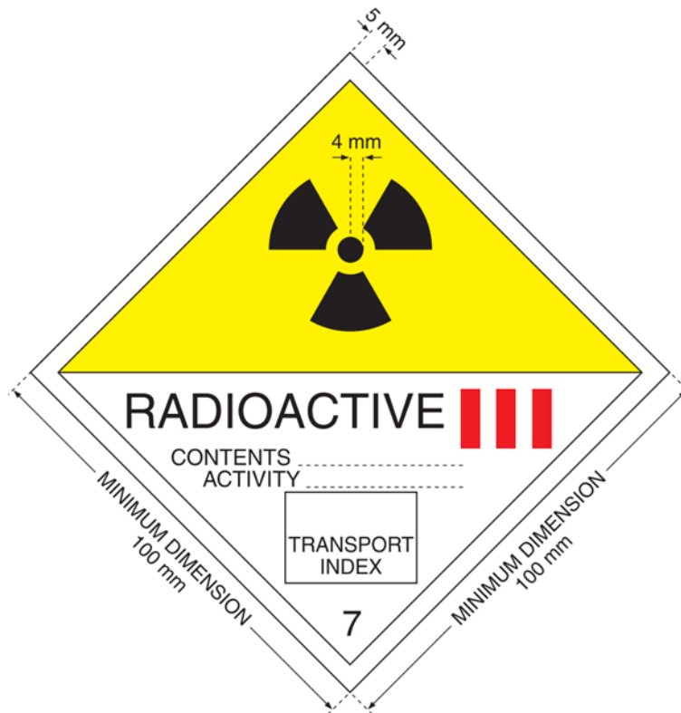
FIG. 4. Category III-YELLOW label. The minimum width of the line inside the edge forming the diamond shall be 2 mm. There shall be a line inside the edge forming the diamond which shall be parallel and approximately 5 mm from the outside of that line to the edge of the label. The background colour of the upper half of the label shall be yellow and the lower half white, the colour of the trefoil and the printing shall be black, and the colour of the category bars shall be red.
