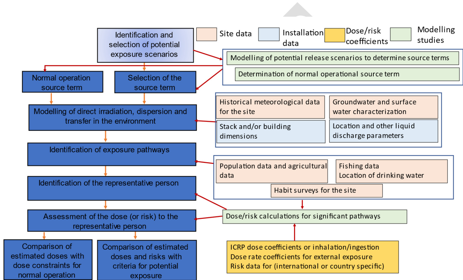
FIG. 1. Data used and modelling performed at the various stages of the radiological environmental impact assessment for normal operation and accident conditions.
