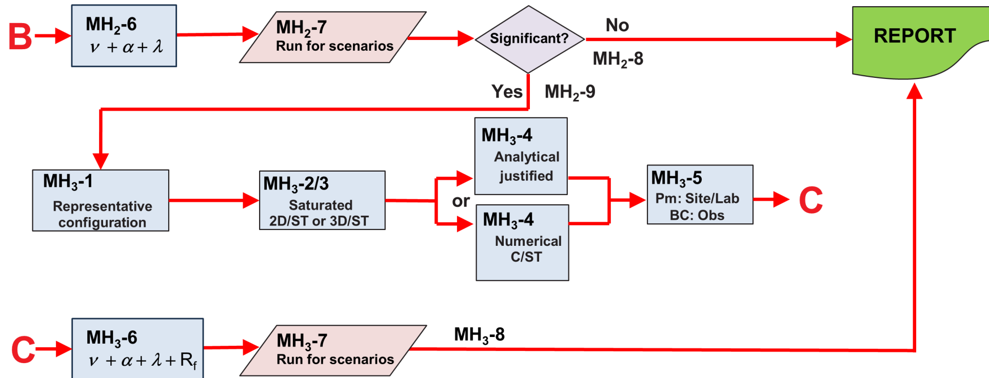
FIG. 6. Flow chart showing a graded approach to modelling radionuclide transfer in groundwater in Reporting Stage 1 of site evaluation for medium hazard category nuclear installations.
