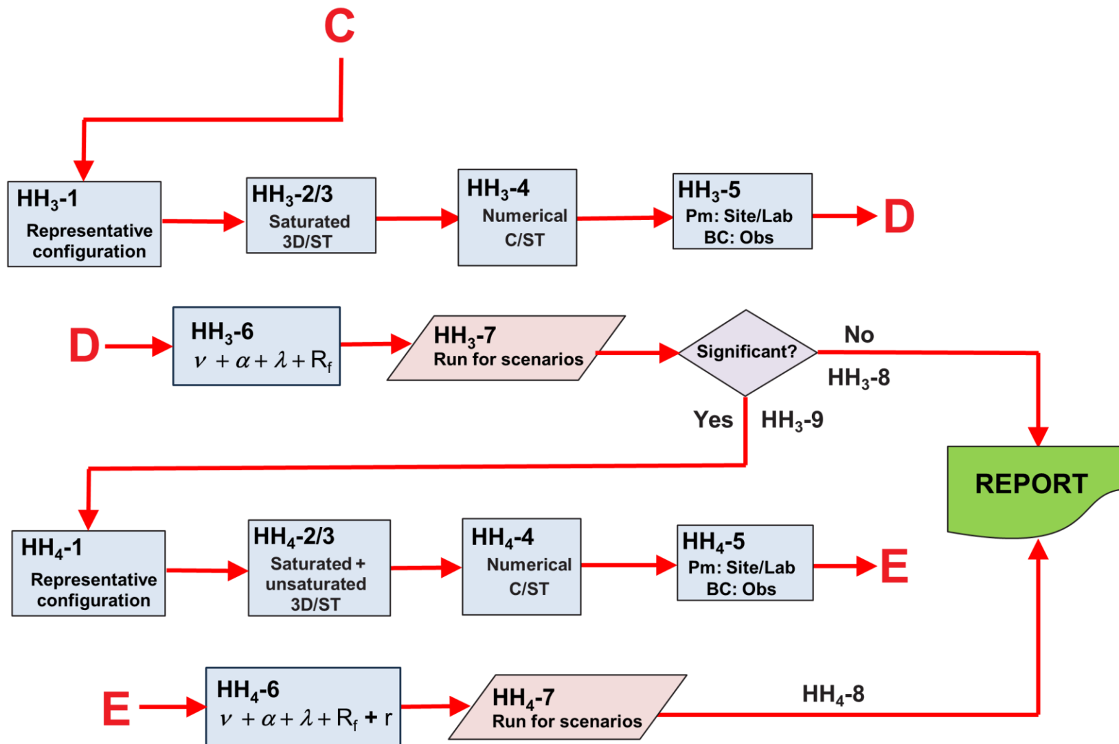
FIG. 7. Flow chart showing a graded approach to modelling radionuclide transfer in groundwater in Reporting Stage 1 of site evaluation for high hazard category nuclear installations.
