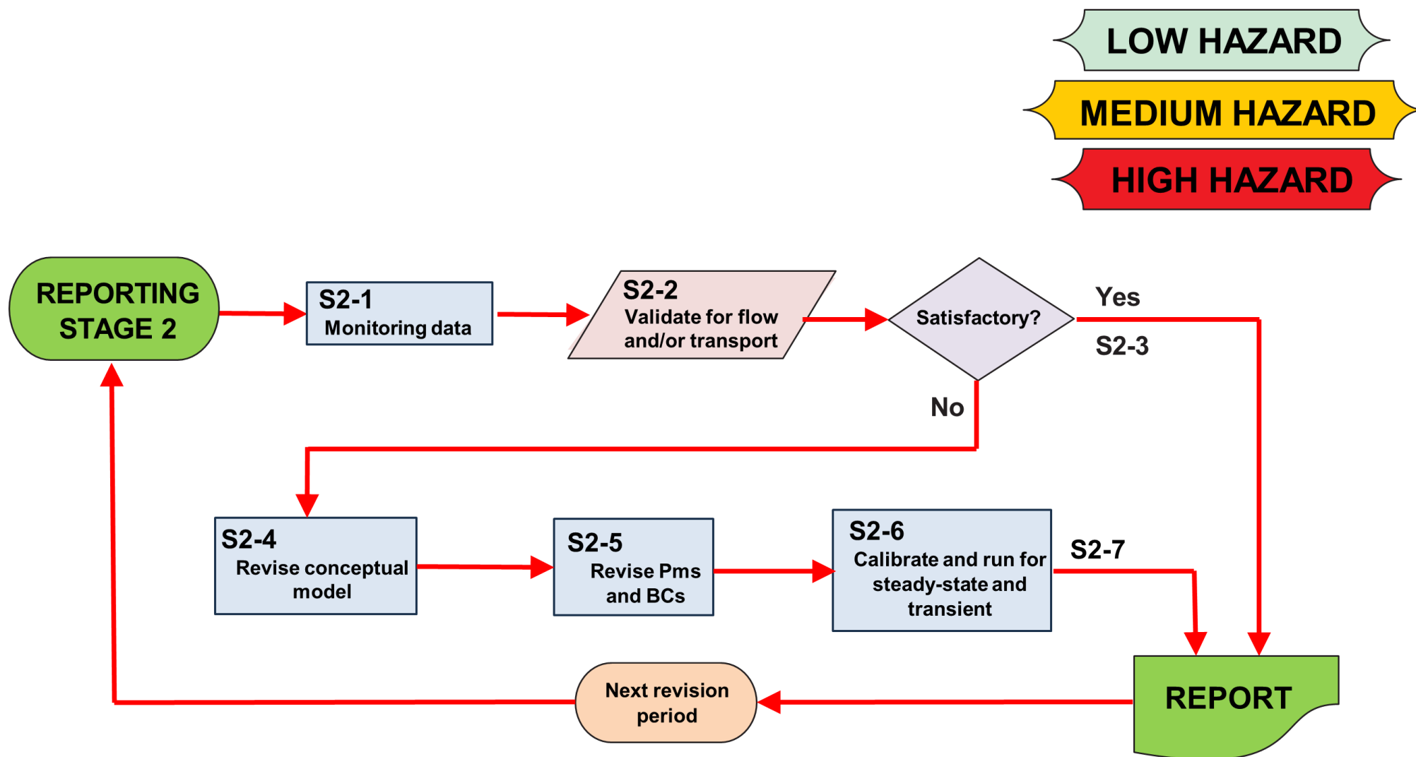
FIG. 8. Flow chart showing steps of modelling radionuclide transfer in groundwater in Reporting Stage 2 of site evaluation for low, medium and high hazard category nuclear installations.
