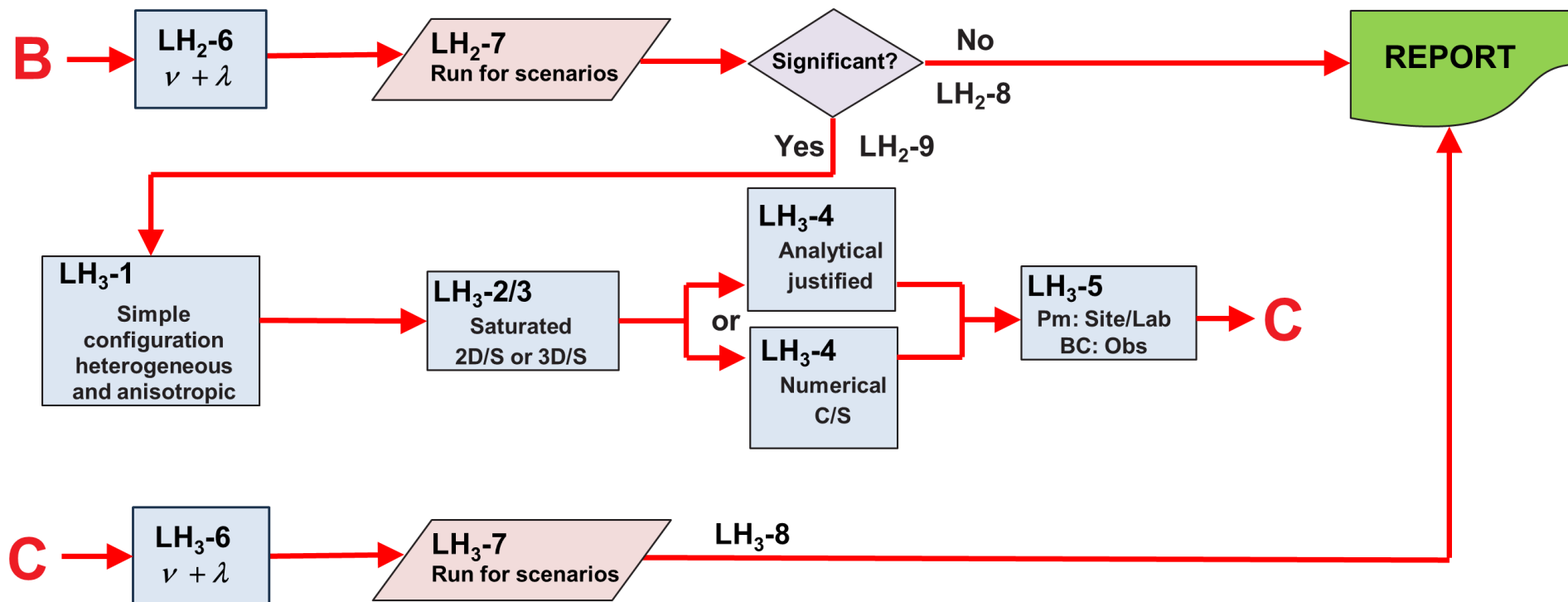
FIG. 5. Flow chart showing a graded approach to modelling radionuclide transfer in groundwater in Reporting Stage 1 of site evaluation for low hazard category nuclear installations.
