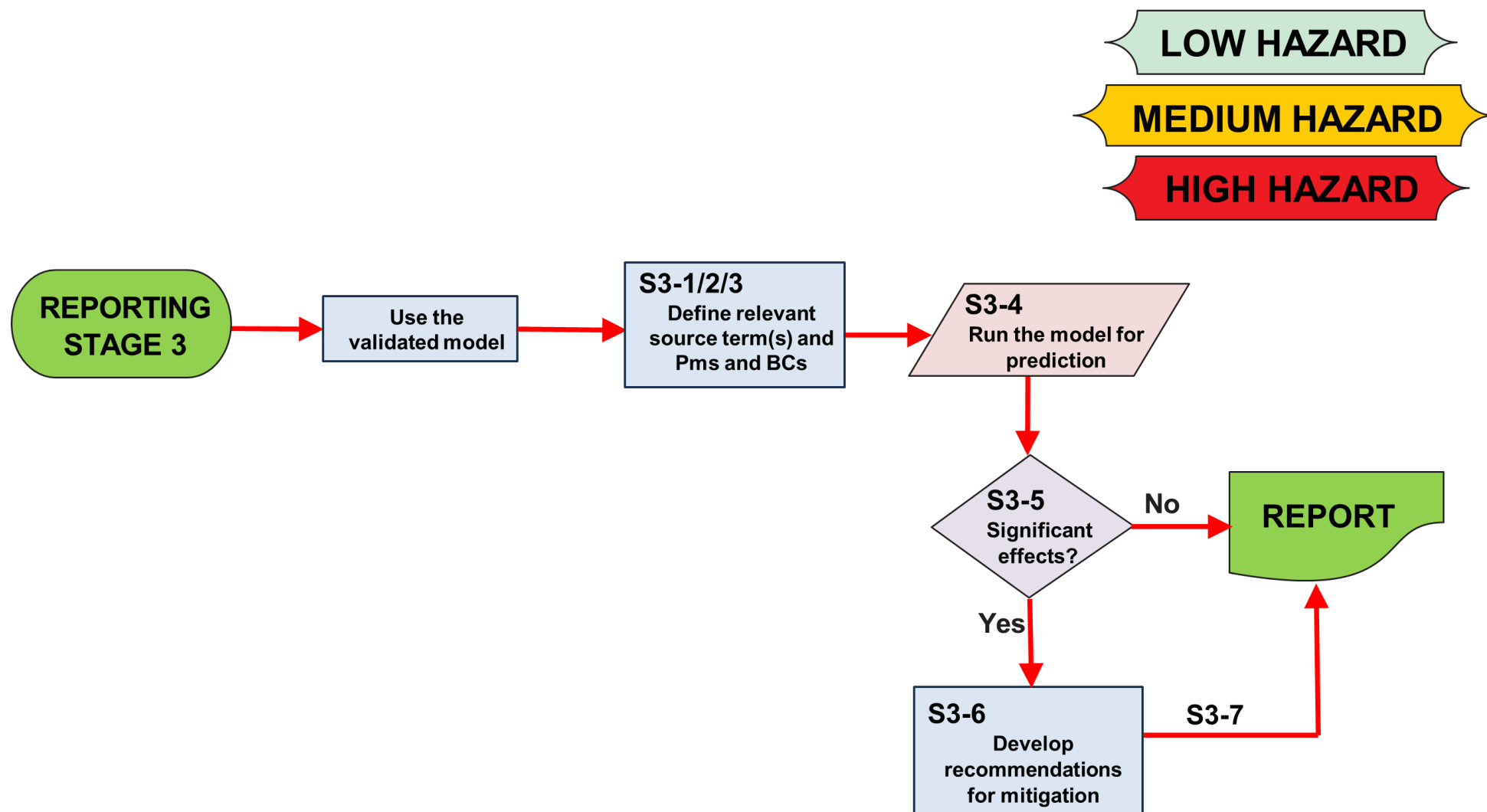
FIG. 9. Flow chart showing steps of modelling radionuclide transfer in groundwater in Reporting Stage 3 of site evaluation for low, medium and high hazard category nuclear installations.
