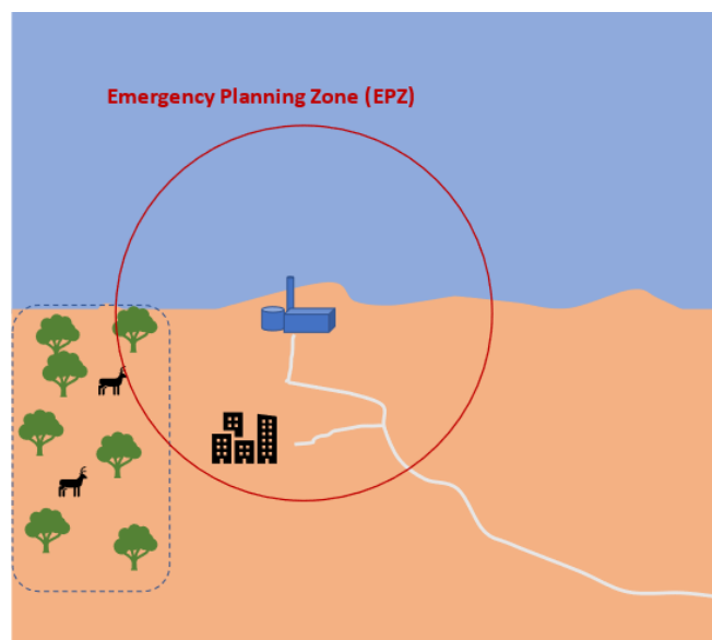
FIG. 3. Example of a site with an administrative barrier (national park or special area) preventing construction of an alternative evacuation route in another direction. The site potentially is unsuitable.
