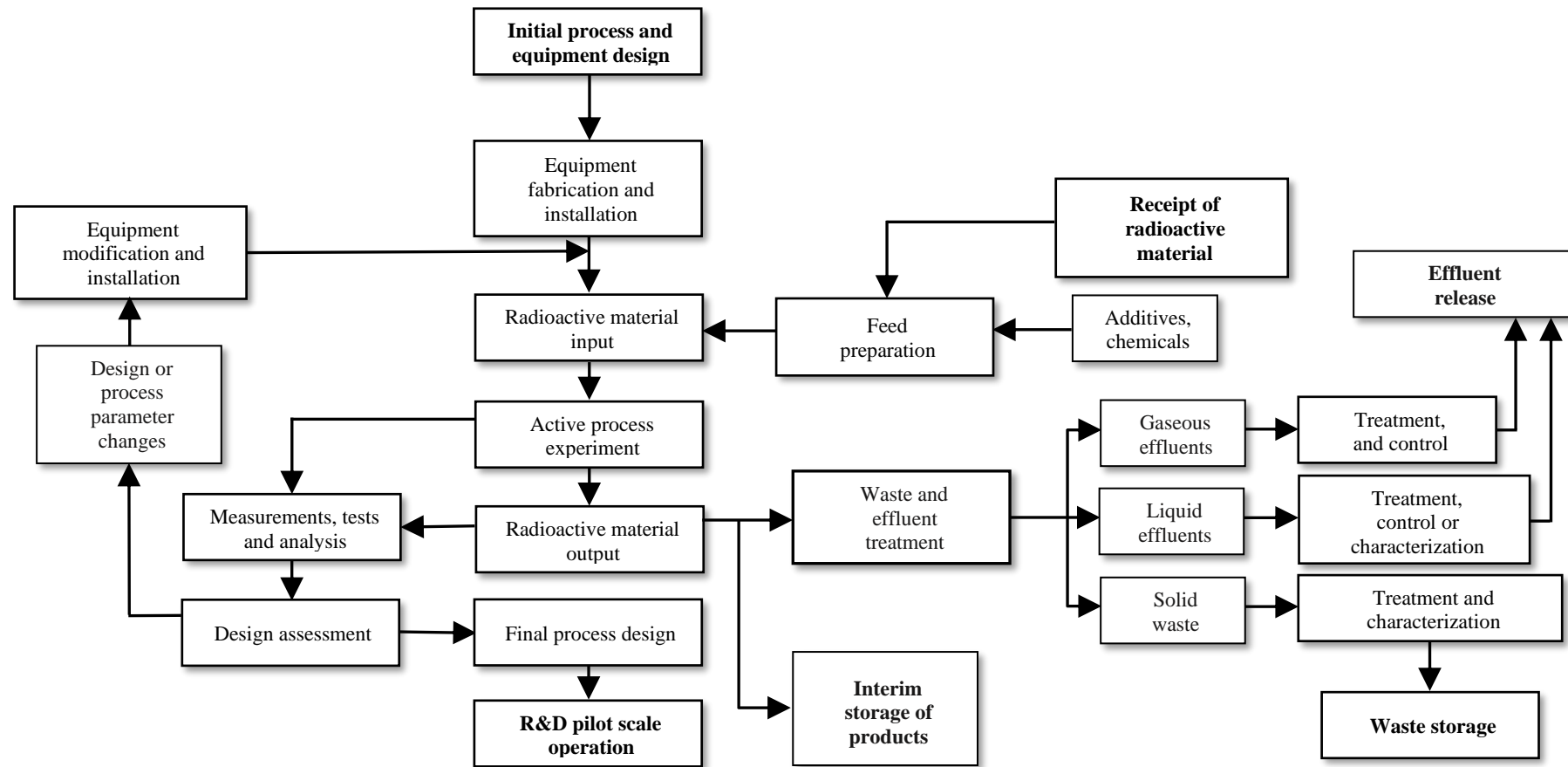
FIG. I-2. Diagram showing the general processes in an nuclear fuel cycle R&D facility operating at a pilot scale (Case 2)
