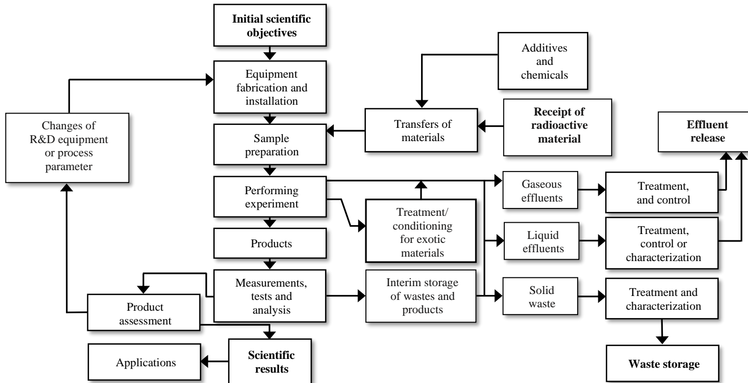
FIG. I-1. Diagram showing the general processes in a nuclear fuel cycle R&D facility operating at laboratory scale (Case 1)
