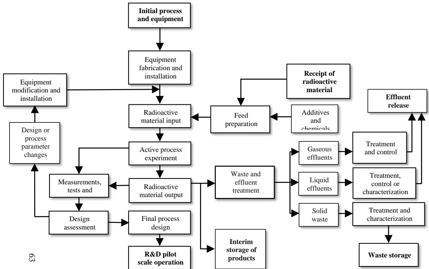
FIG. I-2. Diagram showing the general General processes in ana nuclear fuel cycle R&D facility operating at a pilot scale (Case-2) .
