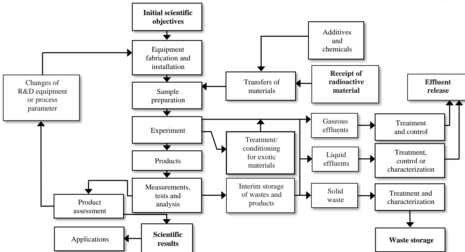
FIG. I-1. General processes in a nuclear fuel cycle R&D facility operating at laboratory scale (Case 1).
