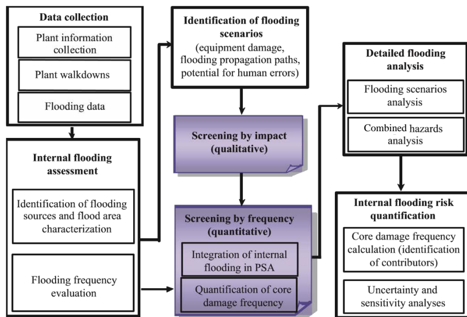
FIG. 4. Process for development of a Level 1 PSA for internal flooding 43
