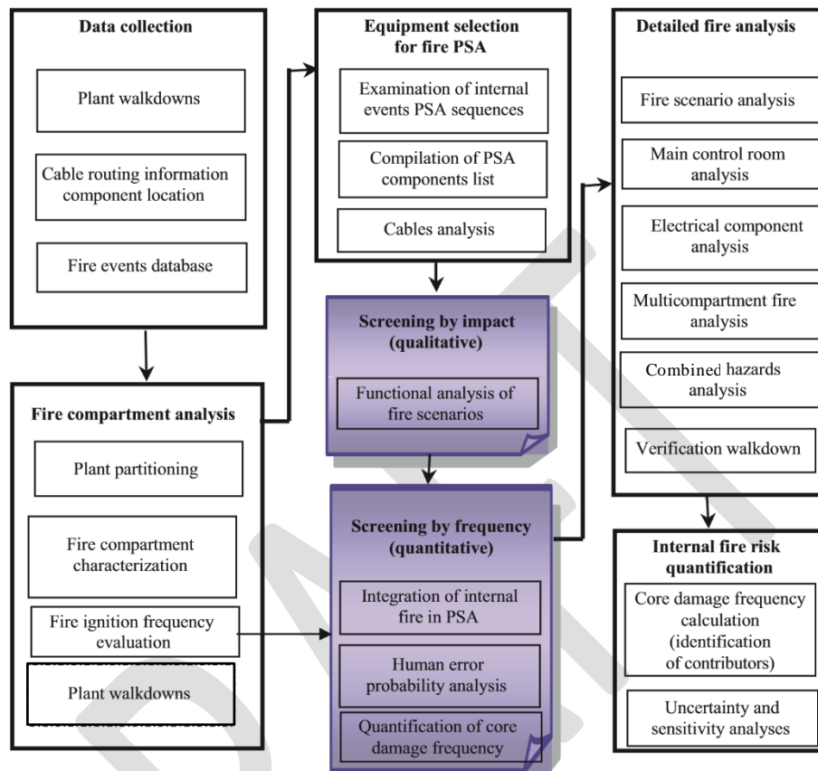
FIG. 3. Process for development of a Level 1 PSA for internal fire 43 .
