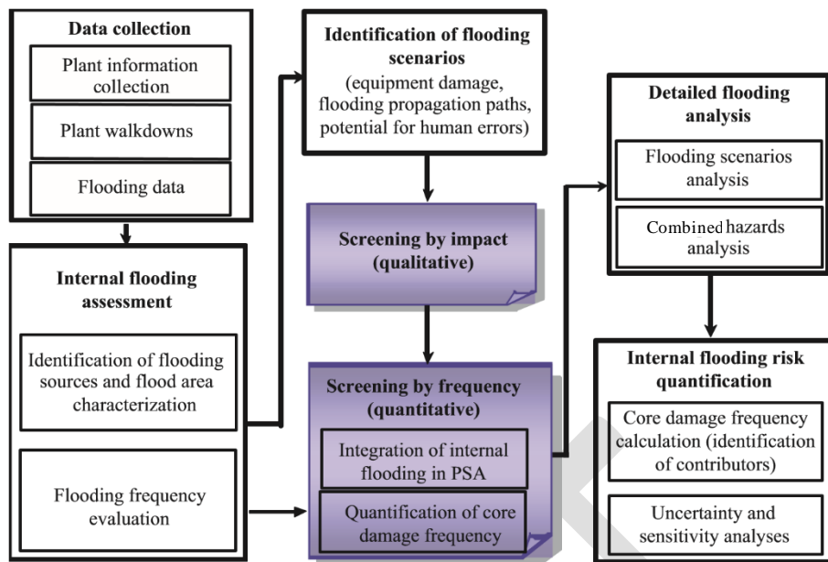
FIG. 4. Process for development of a Level 1 PSA for internal flooding 44
