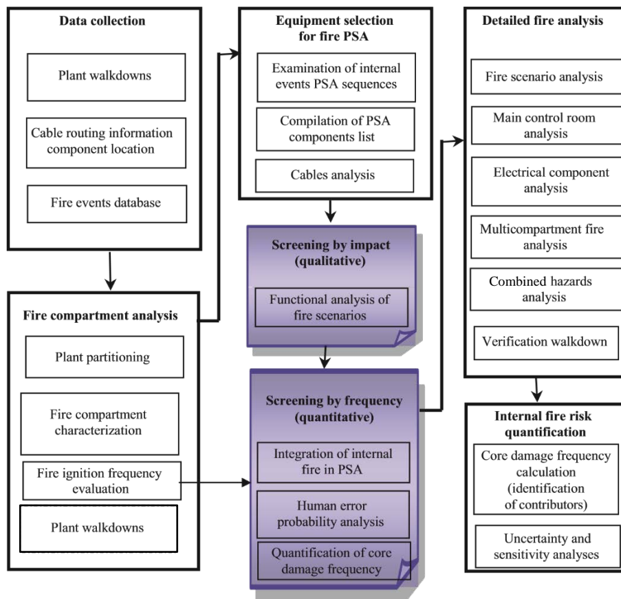
FIG. 3. Process for development of a Level 1 PSA for internal fire 42 .
