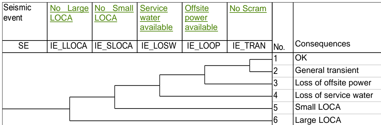
FIG. II-2. Example of an event tree for the modelling of a seismically induced initiating event. LOCA: loss of coolant accident. 77
