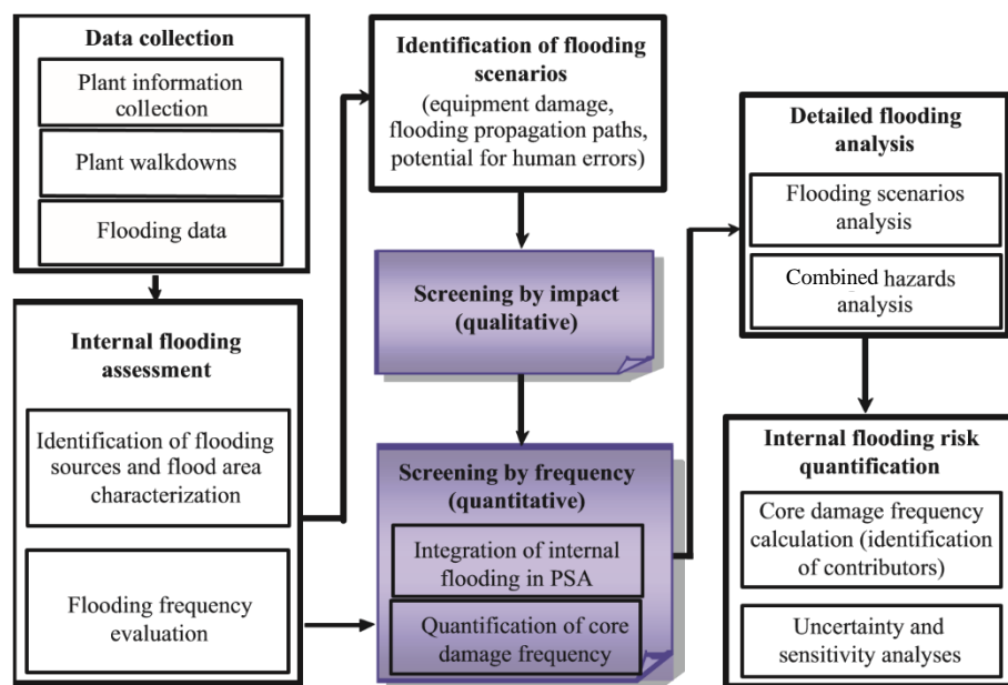
FIG. 4. Process for development of a Level 1 PSA for internal flooding 41
