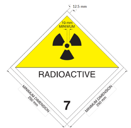
FIG. 6. Placard. Except as permitted by para. 571, minimum dimensions shall be as shown; when different dimensions are used, the relative proportions must be maintained. The number '7' shall not be less than 25 mm high. The background colour of the upper half of the placard shall be yellow and of the lower half white, the colour of the trefoil and the printing shall be black. The use of the word "RADIOACTIVE" in the bottom half is optional, to allow the alternative use of this placard to display the appropriate UN number for the consignment.
