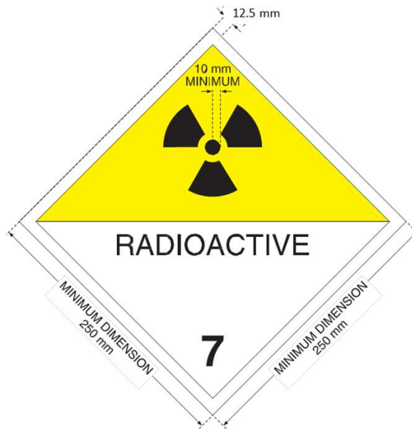
FIG. 6. Placard. Except as permitted by para. 573, minimum dimensions shall be as shown; when different dimensions are used, the relative proportions must be maintained. The number '7' shall not be less than 25 mm high. The background colour of the upper half of the placard shall be yellow and of the lower half white, the colour of the trefoil and the printing shall be black. The use of the word "RADIOACTIVE" in the bottom half is optional, to allow the alternative use of this placard to display the appropriate UN number for the consignment.
