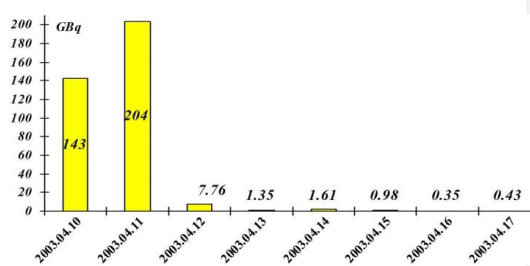
Fig. I-8. I-131 equivalent release.
