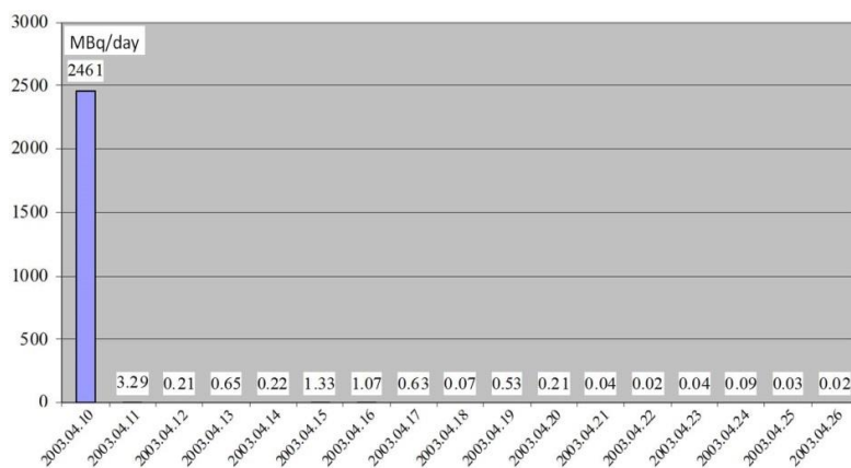
Fig. I-9. Airborne release.
