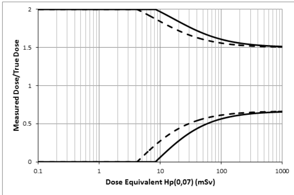
FIG. 4. Acceptable upper and lower limits for the ratio measured dose/conventional true dose as a function of dose: (a) for H_p(10) ; and (b) for H_p(0.07) . (Broken lines: monthly monitoring periods; solid lines: two-month monitoring periods.)
