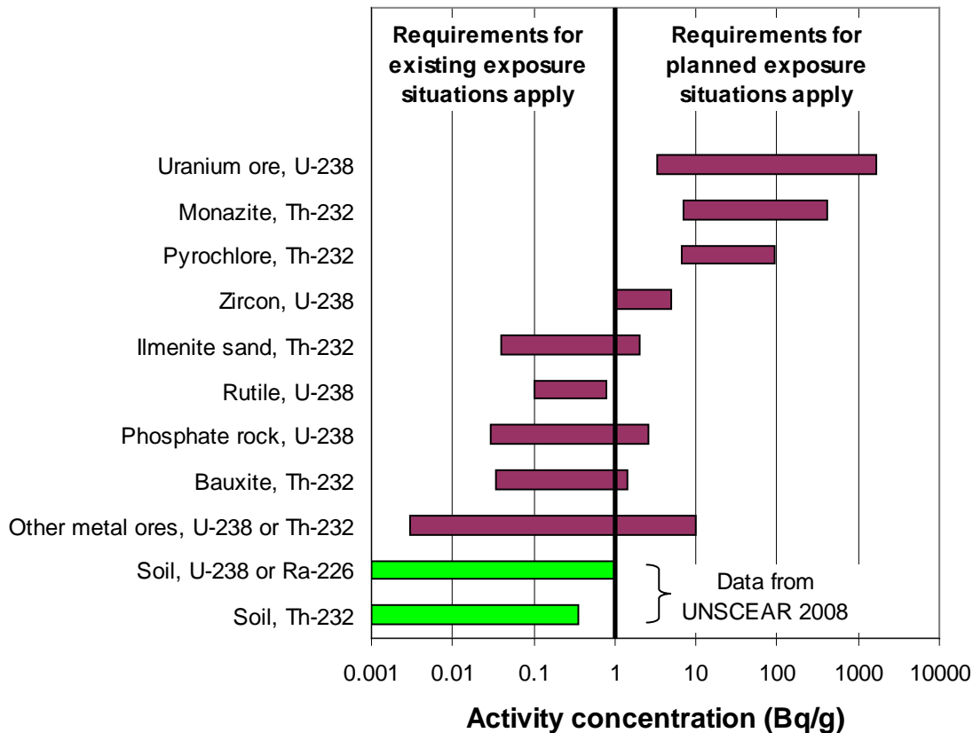
FIG. 3. Radionuclide activity concentrations in natural materials.
