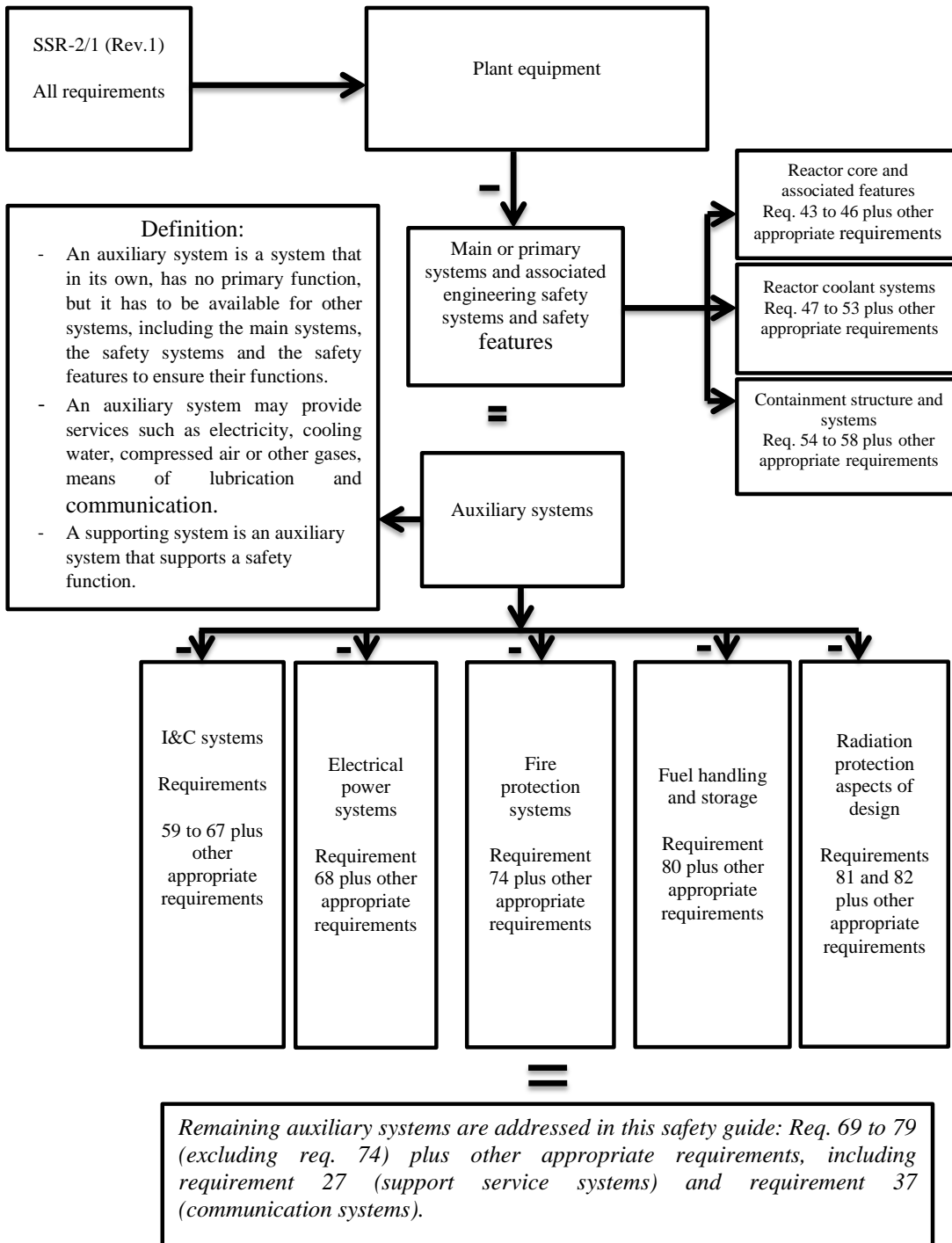
Figure 1. Stepwise approach to define the addressed auxiliary systems and supporting systems AS&SS
