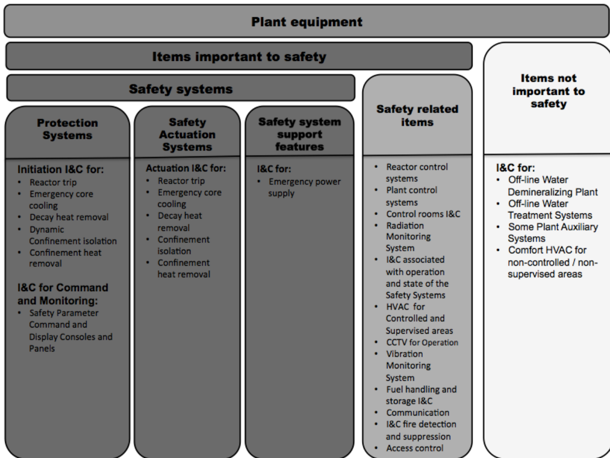
FIG. 1. Examples of instrumentation and control systems of a research reactor classified according to their importance to safety. (See also Annex I.)
