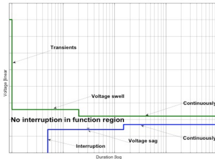
FIG. 65. Voltage swell and sag (note that initial conditions could be anywhere within the continuous band).
