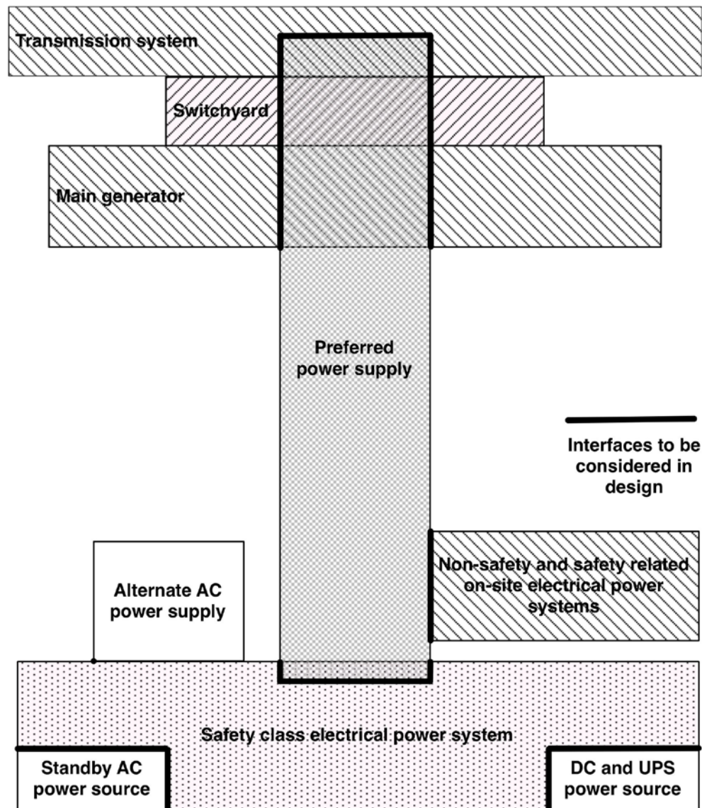
FIG. 54. Relationship between the preferred power supply and other elements of the electrical power system.
