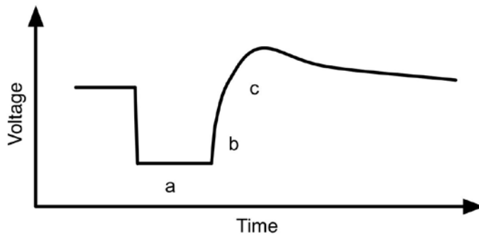
FIG. 76. Typical on-site voltage profile during clearing of transmission system fault, a. Voltage during fault, b. Rapid voltage rise, c. Voltage swell due to generator excitation and return to normal voltage.
