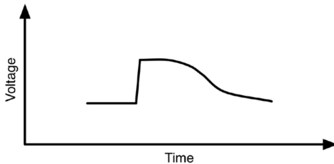
FIG. 87. Typical on-site voltage profile after loss of load (transfer to house load operation).
