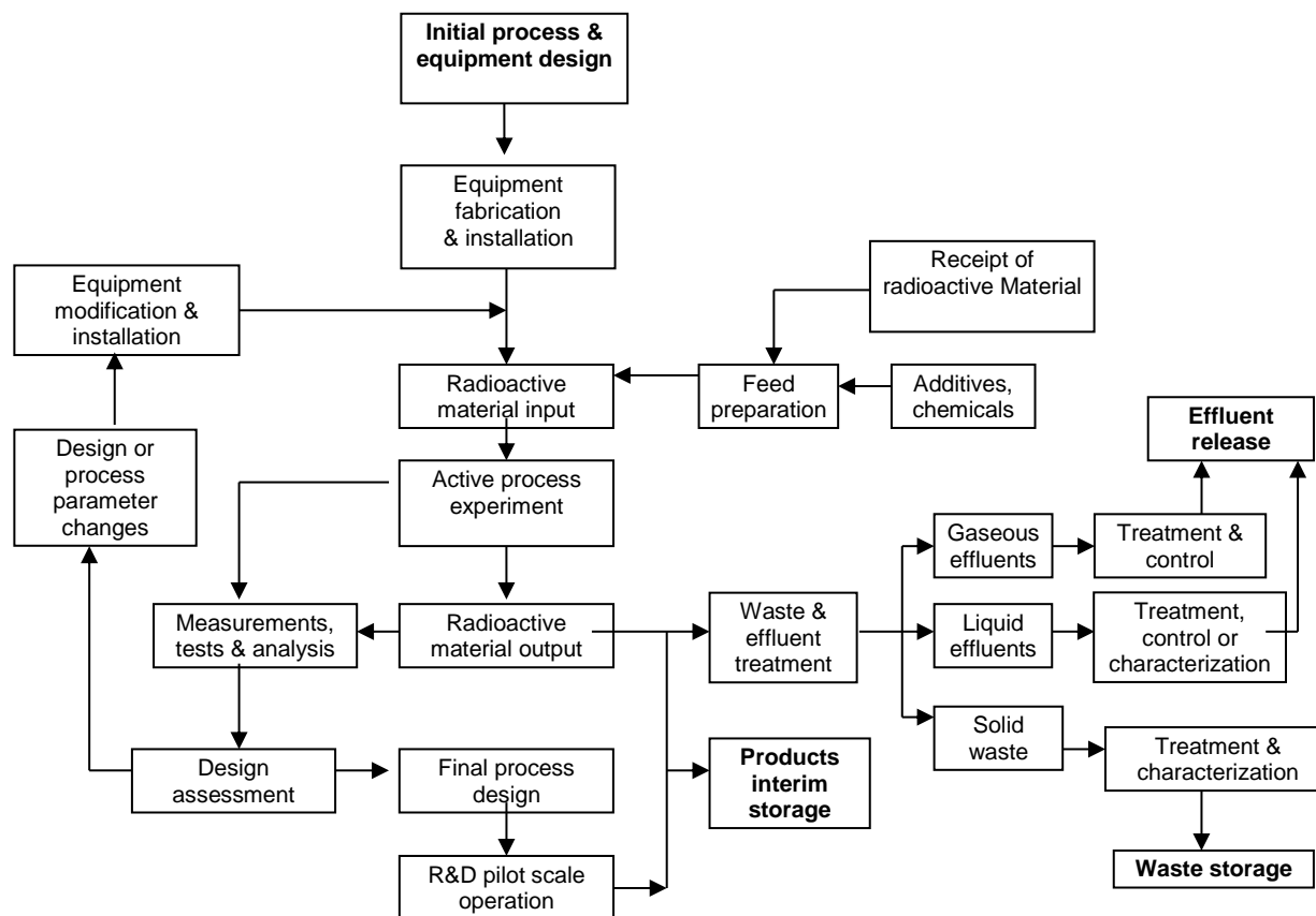
FIG. II-1. Diagram showing the general processes in an R&D facility operating at a pilot scale (case 2).
