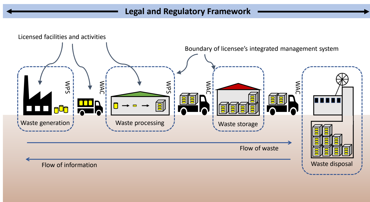
FIG. 1 Illustration of the Systemic Control systemic control of Radioactive Waste Management radioactive waste management by Operating Organizations operating organizations at Different Facilities different facilities working under a series of Management Systems management systems . WPS: waste package specifications; WAC: waste acceptance criteria.
