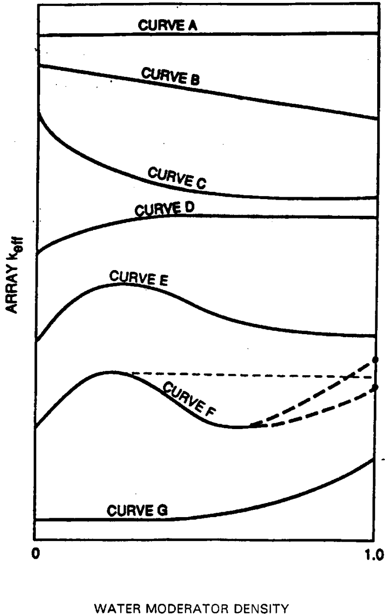
FIG. VI.1. Typical plots of array k_{eff} versus interspersed water moderator density.
