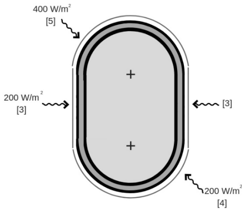
FIG. 6. Vertical cross-section of package with curved surfaces ([3–5] denotes cases as shown in Table 12 of the Transport Regulations).
