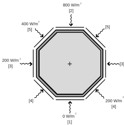
FIG. 5. Horizontal cross-section of package with flat surfaces ([1–5] denotes cases as shown in Table 12 of the Transport Regulations).
