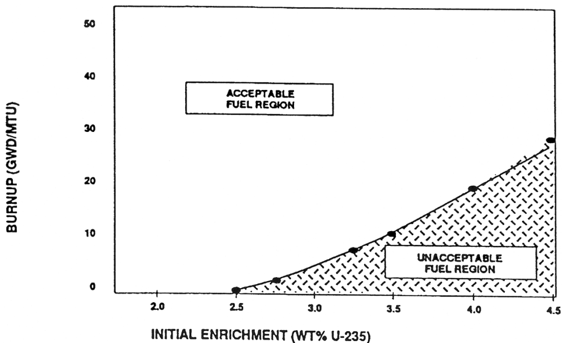
FIG. VI.2. Loading curve indicating the region of burnup and initial enrichment that ensures subcriticality.
