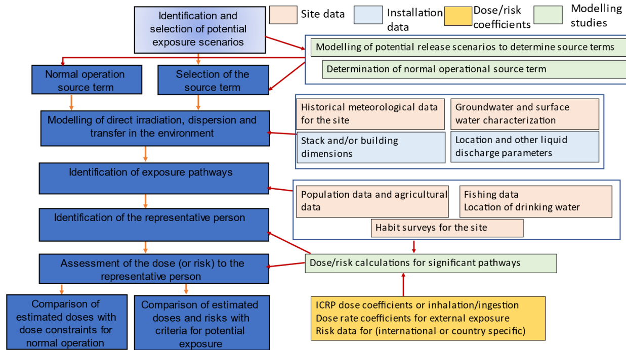
FIG. 1. Data used and modelling performed at the various stages of radiological environmental impact assessment for normal operation and accident conditions.
