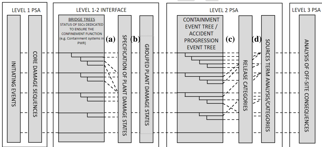
FIG. 1. General overview of the development of a typical Level 2 PSA.
