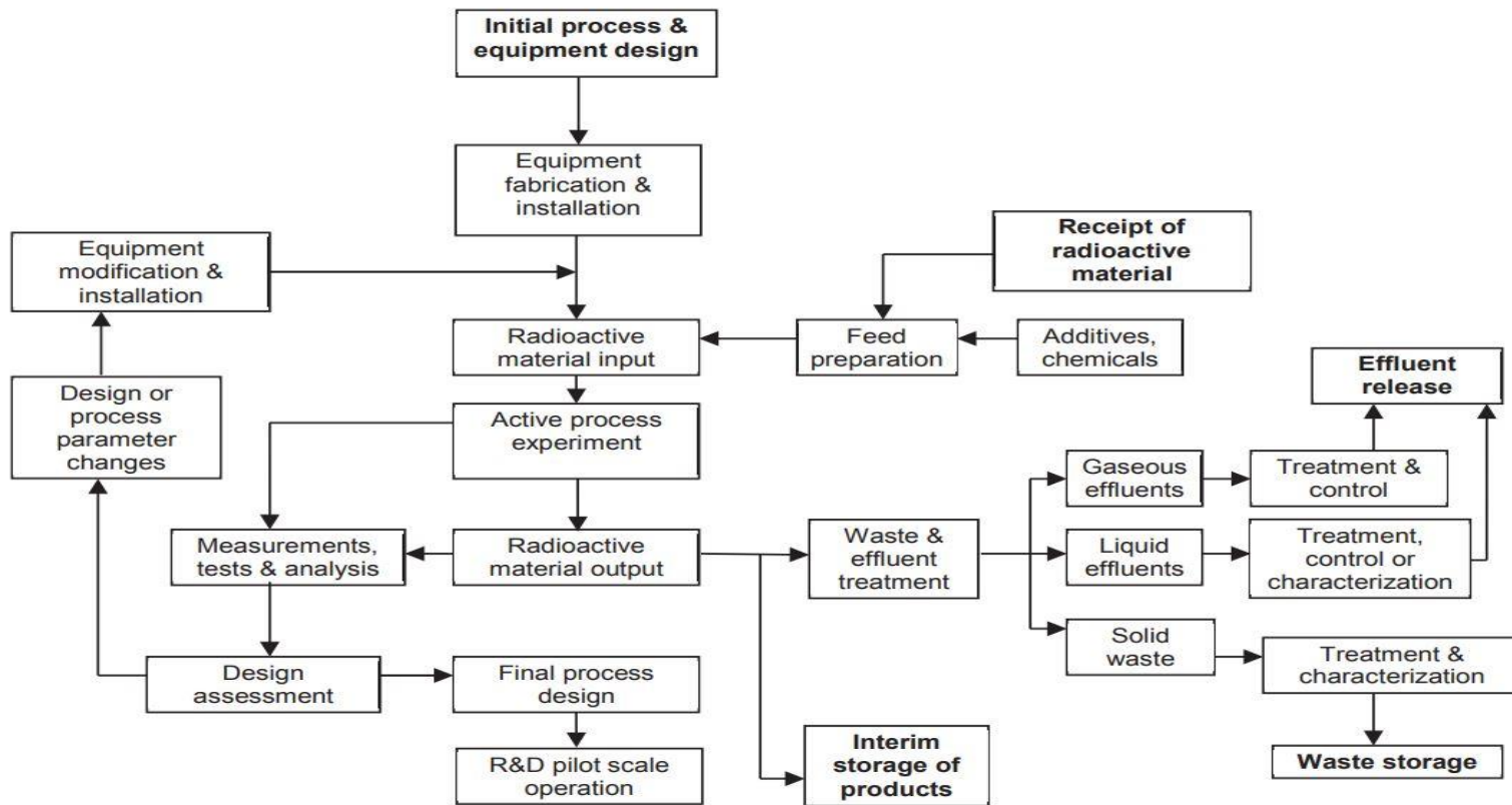
FIG. I-2. Diagram showing the general processes in an nuclear fuel cycle R&D facility operating at a pilot scale (Case 2)
