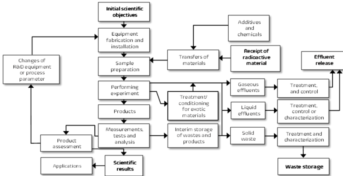
FIG. I-1. Diagram showing the general processes in an a nuclear fuel cycle R&D facility operating at laboratory scale (Case 1)
